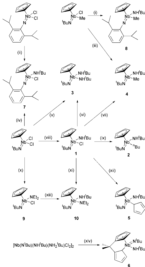
Scheme 1 Reagents and conditions: (i) LiNH(2,6-C 6 H 3 Pr 2 ), Et 2 O, –78 °C. (ii) LiNH t Bu, C 6 H 6 . (iii) LiNH t Bu, C 6 H 6 . (iv) LiNH(2,6-C 6 H 3 Pr 2 ), Et 2 O, –78 °C. (v) 2 LiNH t Bu, C 6 H 6 . (vi) LiNH t Bu, C 6 H 6 . (vii) LiMe, Et 2 O, –78 °C. (viii) LiNH t Bu, C 6 H 6 . (ix) n BuLi, C 5 H 12 , –78 °C. (x) LiNEt 2 , Et 2 O, –78 °C. (xi) LiNEt 2 , Et 2 O, –78 °C. (xii) Mg(C 5 H 5 ) 2 , C 6 H 6 . (xiii) LiNH t Bu, C 6 H 6 . (xiv) Li 2 {(C 5 H 4 ) 2 CM 2 }, THF, –78 °C.
